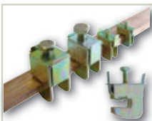
Branching-off terminals for collecting rails (buses) 18
