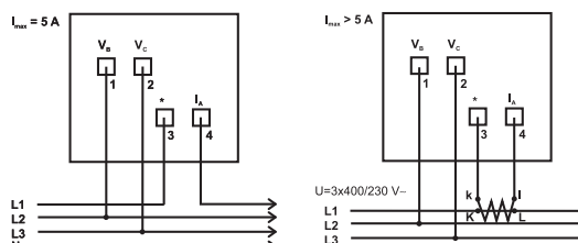
Wiring diagram for three phases system
