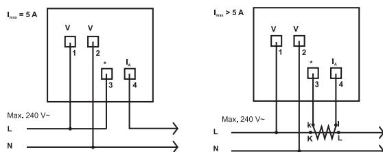
Wiring diagram for one phase system
